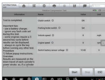
RELATIVE COMPRESSION
